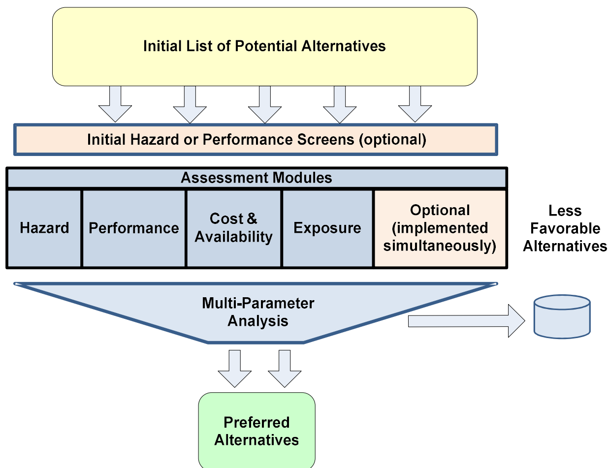
Figure 7: Simultaneous Framework.
