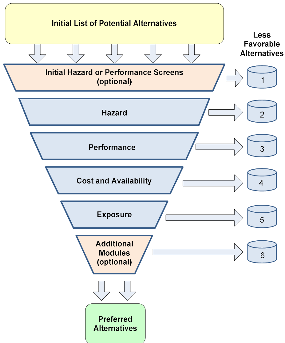
Figure 5: Sequential Framework.
